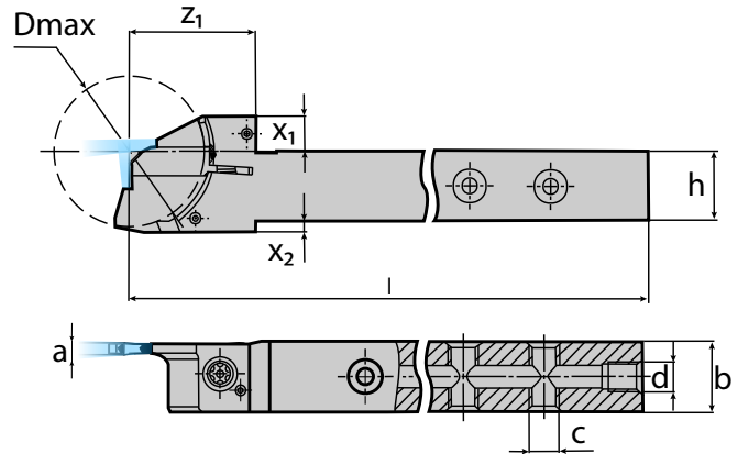
Tool Holders with coolant IC+ (IC-Plus)
